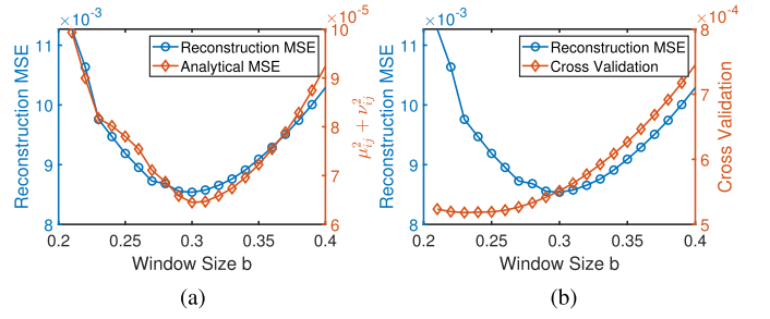
Fig. 2. (a) The MSE of the propagation map reconstruction and the analytical MSE of the interpolation based on (21); the minimizers \hat{b} are matched; (b) The MSE of the propagation map reconstruction and the cost from cross validation based on (20); the minimizers \hat{b} are mismatched.
