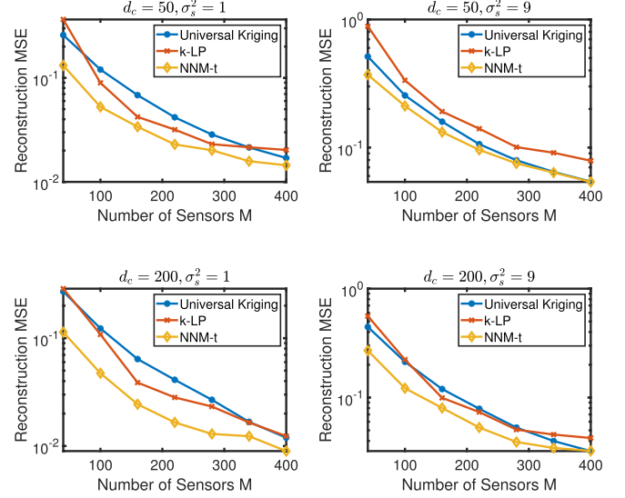
Fig. 6. Performance under different shadowing parameters.
