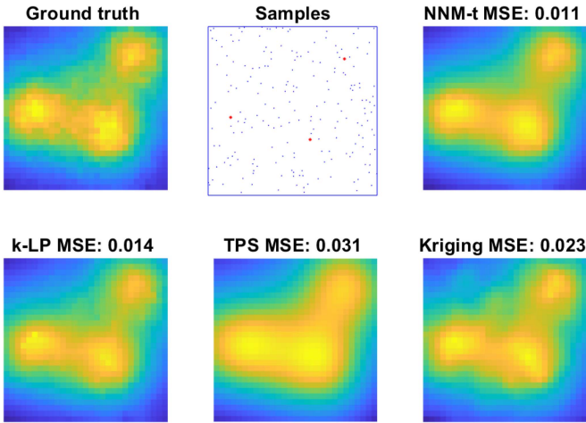
Fig. 8. Ground truth, sampling pattern, and the reconstruction MSE of different methods.
