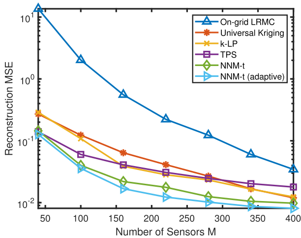
Fig. 7. Reconstruction MSE for S = 3 and N = 30 .
