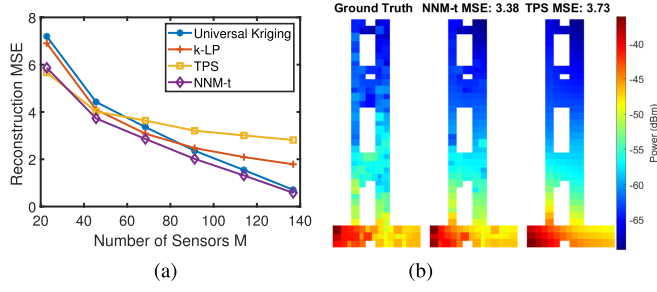
Fig. 10. The reconstruction performance evaluated on real data set. (a) The reconstruction MSE versus the number of measurements used for propagation map construction. (b) Visualization of the propagation field in an indoor environment, showing the ground truth, the reconstruction from NNM-t, and the reconstruction from TPS.
