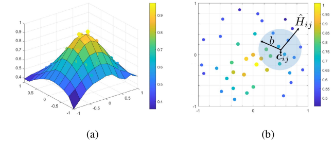
Fig. 1. (a) Propagation map reconstruction based on local polynomial regression (b) Sensor measurements (colored dots) within a range of b (grey region) from the grid center \mathbf{c}_{ij} are used to estimate \hat{H}_{ij} .
