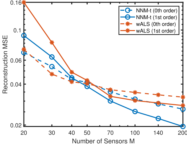
Fig. 5. Reconstruction MSE for S = 1 and N = 30 . Zeroth order interpolation performs better for a small number sensors, whereas, first order method prefers more sensors.
