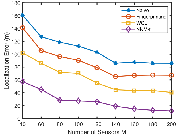
Fig. 9. Source localization error for S = 1 and N = 30 .
