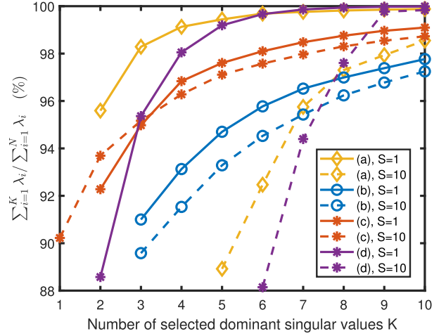
Fig. 3. Percentage of the sum of the first K dominant singular values over the sum of all singular values for a 100 by 100 propagation matrix.
