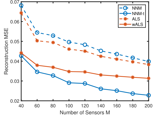
Fig. 4. Reconstruction MSE for S = 1 and N = 30 . The uncertainty-aware scheme works.
